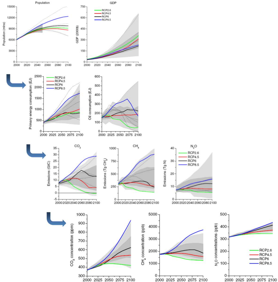
Figure 4: Socioeconomic (top row), energy intensity (second row), greenhouse gas emission (third row), and ultimately greenhouse gas concentration (bottom row) assumptions underlying the representative concentration pathways (RCPs) used to drive future climate projections. From van Vuuren, et al., 2011, reproduced with permission.
