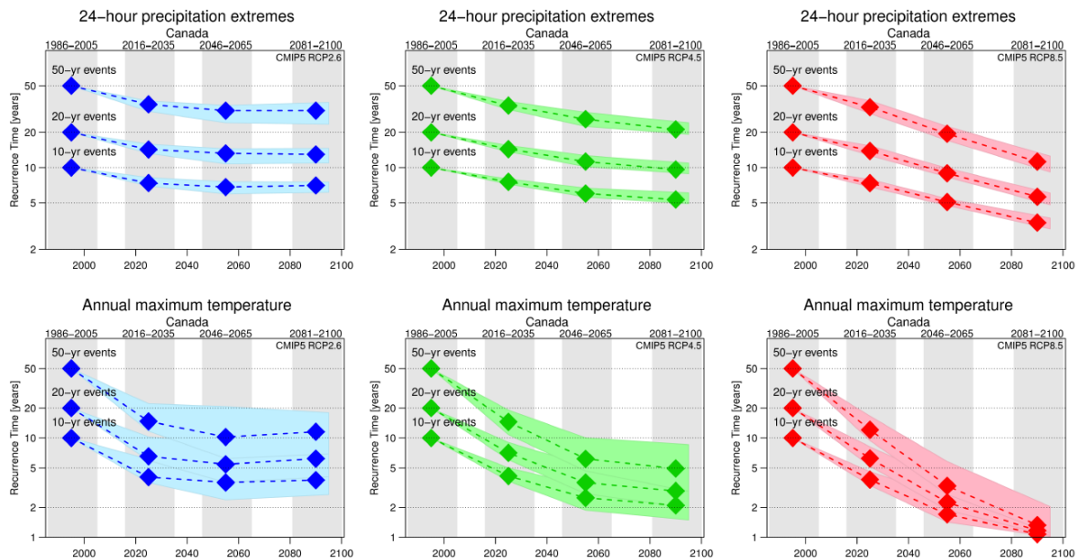
Figure 11: Projected return periods (in years) for late-twentieth century 10-, 20-, and 50-year return values of annual maximum 24-hour precipitation (upper panel) and annual maximum temperature (lower panel) over Canada as simulated by GCMs contributing to the CMIP5 for three RCPs (RCP2.6, left; RCP4.5, middle; RCP8.5, right). Values are computed based on Kharin et al., 2013.
