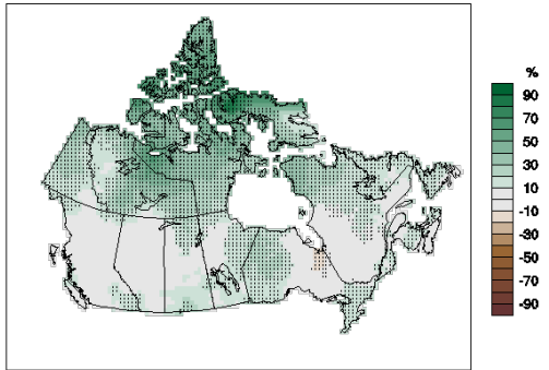
Annual total precipitation trends 1900-2012
