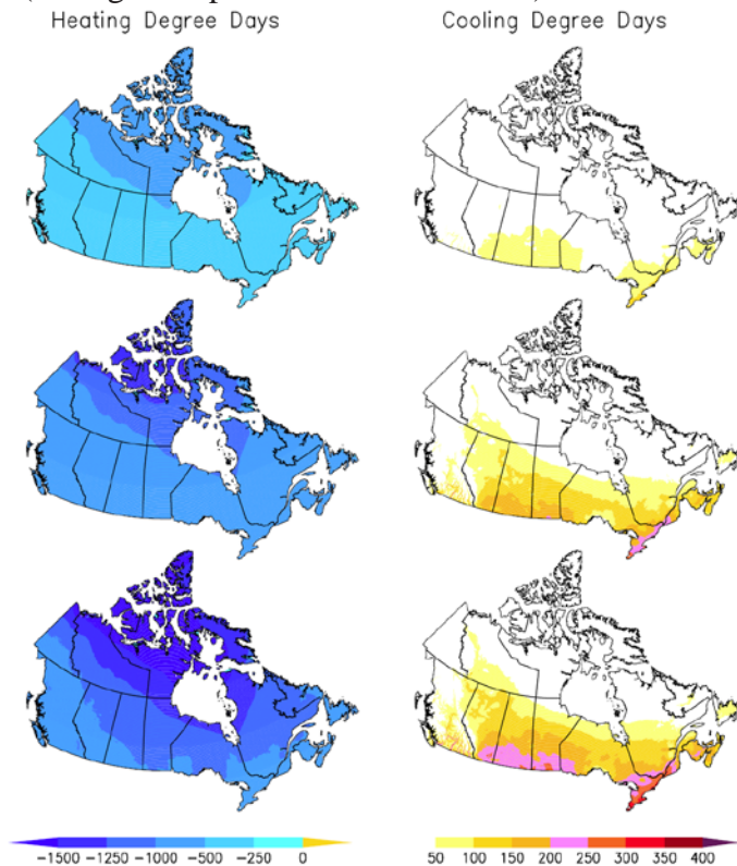
Figure 14: Illustration of potential utility of statistically downscaled projections of extremes. Projected changes in heating (left panel) and cooling (right panel) degree days (in degree-days) are shown for the 2016–2035 (top), 2046–2065 (middle), and 2081–2100 (bottom) periods. Projected changes are relative to the 1986–2005 mean estimated from the multi-model ensemble shown in Table 7 and downscaled using BCCAQ.
