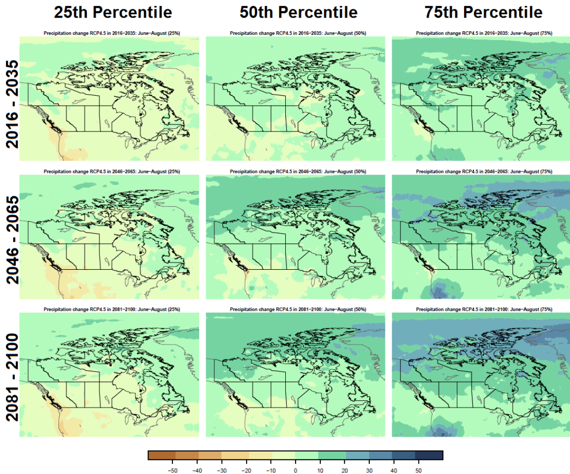
Figure 10: Maps of summer precipitation change projected by the CMIP5 multi-model ensemble for the RCP4.5 scenario, averaged over June–August. Change is computed relative to the 1986–2005 baseline period. As in the IPCC Atlas (IPCC, 2013), the top row shows results for the period 2016–2035, the middle row for 2046–2065, and the bottom row for 2081–2100. For each row the left panel shows the 25 th percentile, the middle panel the 50 th percentile (median), and the right panel the 75 th percentile. The colour scale indicates precipitation change in % with positive change (increased precipitation) indicated by green colours and decrease by yellow to brown colours, consistent with the colour scale used in the IPCC AR5 Annex I (IPCC, 2013).
